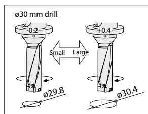
Diameter adjustment range (mm)
