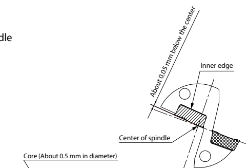
#5 Front view of the drill
