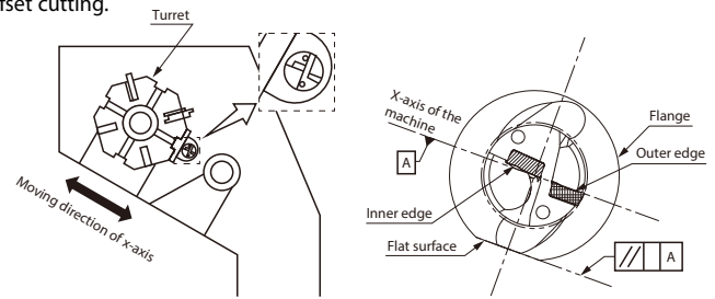
#1 Installed into the lathe
