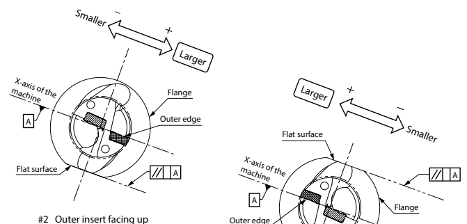
#2 Outer insert facing up
