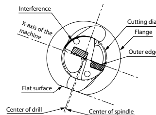
#4 Excessive offset (For smaller hole diameter)
