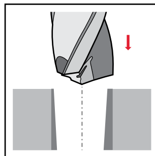
Precast holes
